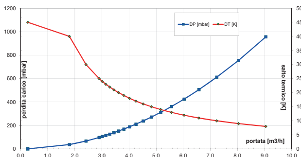
Modula Power II 85
