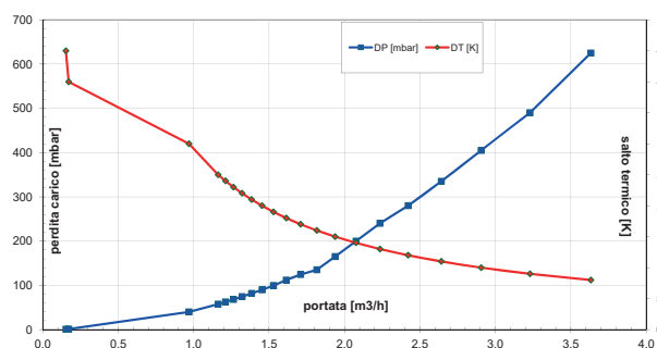
Modula Power II 35 - 45
