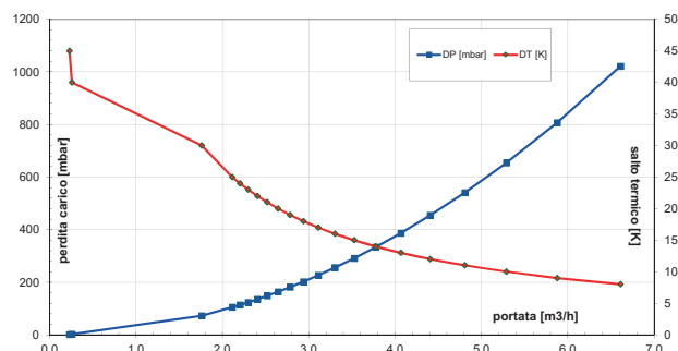
Modula Power II 65
